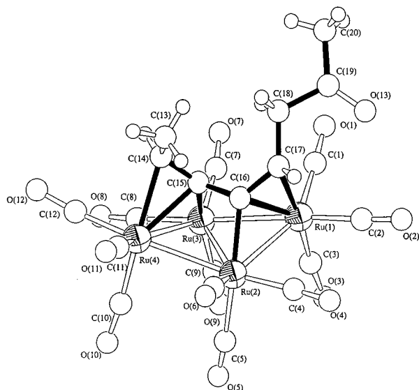
Fig. 1 Molecular structure of [Ru 4 (CO) 12 { \mu_4 - \eta^1 : \eta^1 : \eta^2 -CH 3 C(H)CCC(H)CH 2 C(O)CH 3 }] 1 with the atom numbering scheme.
