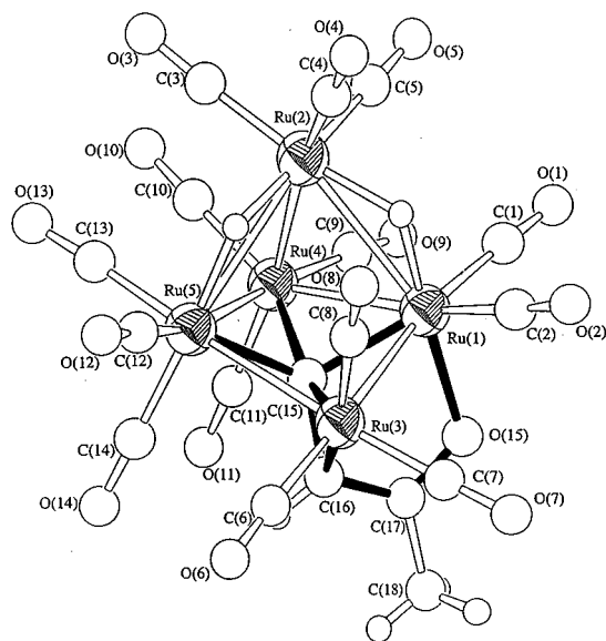
Fig. 2 Molecular structure of [Ru 5 (CO) 14 ( \mu -H) 2 { \mu_4 - \eta^1 : \eta^1 : \eta^2 -CC(H)C(O)CH 3 }] 2 with the atom numbering scheme.
